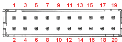
Signal Output Signal Connectors (SK2) JST: PN PHDR-20VS housing and PN: SPHD-001T-P0.5
