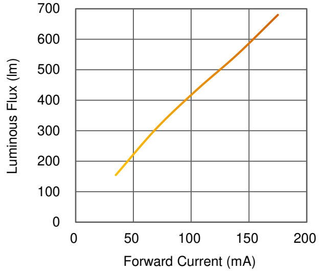
Fig 2. Forward Current vs. Relative Luminous Flux at T C =25°C.
