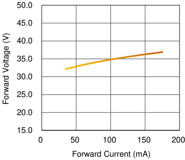
Fig 1. Forward Current vs. Forward Voltage at T C =25°C.
