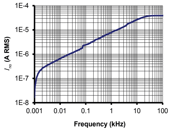
Figure 14: Typical total output RMS noise current with R_M = 50 \Omega ( f_c is upper cut-off frequency of bandpass, low cut off frequency is 1 Hz)
