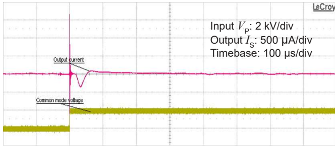
Figure 11: Typical common mode perturbation (2000 V step with 6 kV/μs R_M = 100 \Omega )
