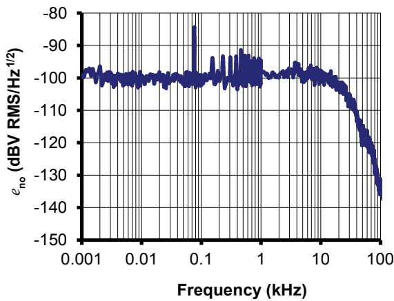
Figure 13: Typical output noise voltage spectral density e_{no} with R_M = 50 \Omega
