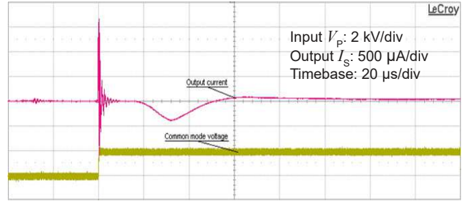
Figure 12: Detail of typical common mode perturbation (2000 V step with 6 kV/μs, R_M = 100 \Omega )
