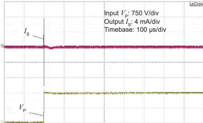
Figure 11: Typical common mode perturbation (1500 V step with 6 kV/ \mu s, R_M = 100 \Omega )
