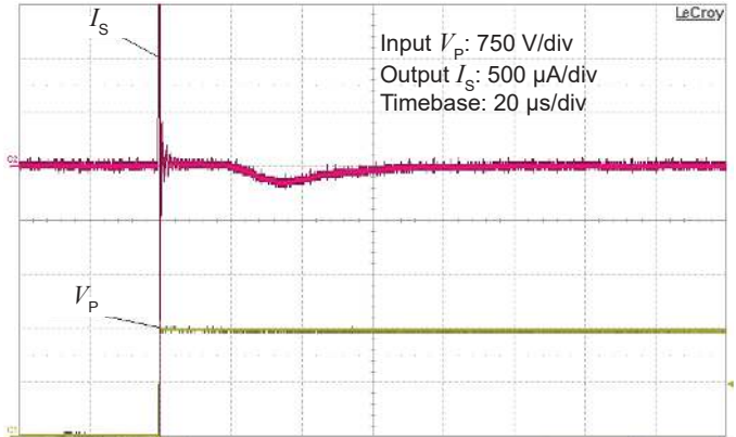
Figure 12: Detail of typical common mode perturbation (1500 V step with 6 kV/ \mu s, R_M = 100 \Omega )
